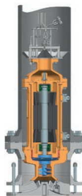
Removable Pump In tank vertical or horizontal
