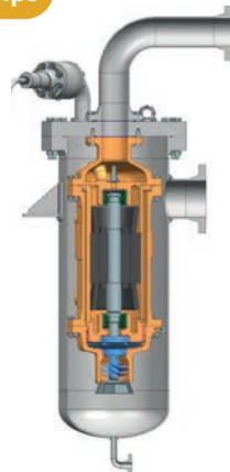
Low pressure Barrel In sump vertical
