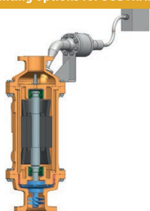
Flanged Version In line vertical or horizontal
